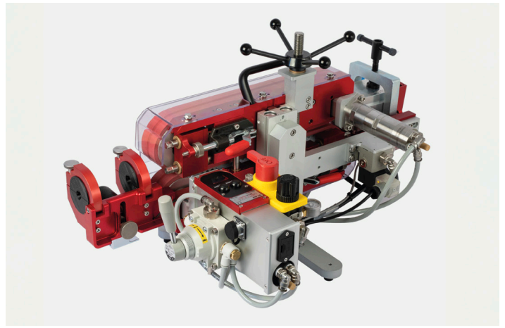
V3 Fiber Blowing Machine
