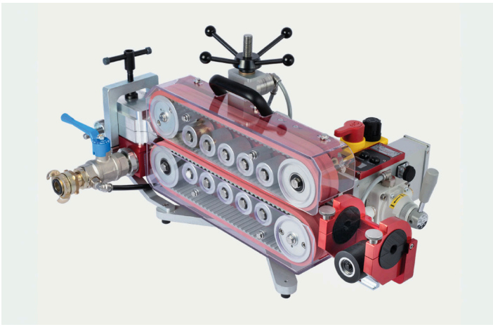
V3 Fiber Blowing Machine
