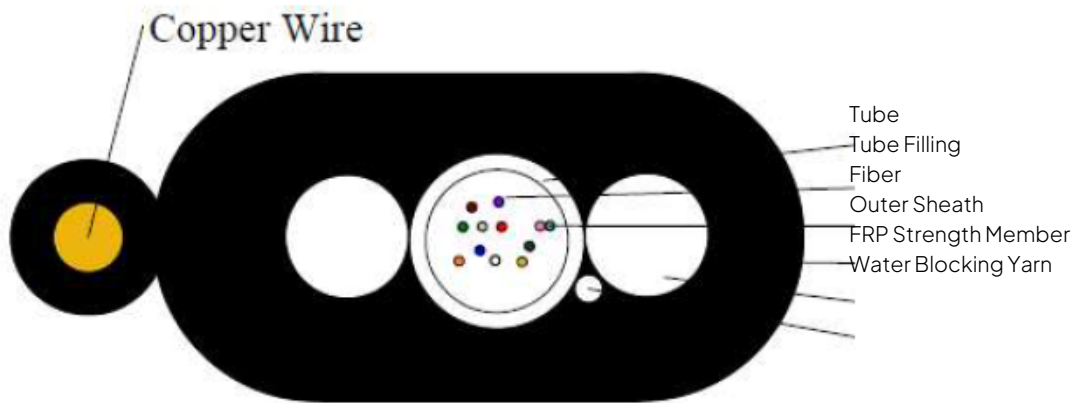
10-11021.01A - 12F Flat Drop Toneable Cable
