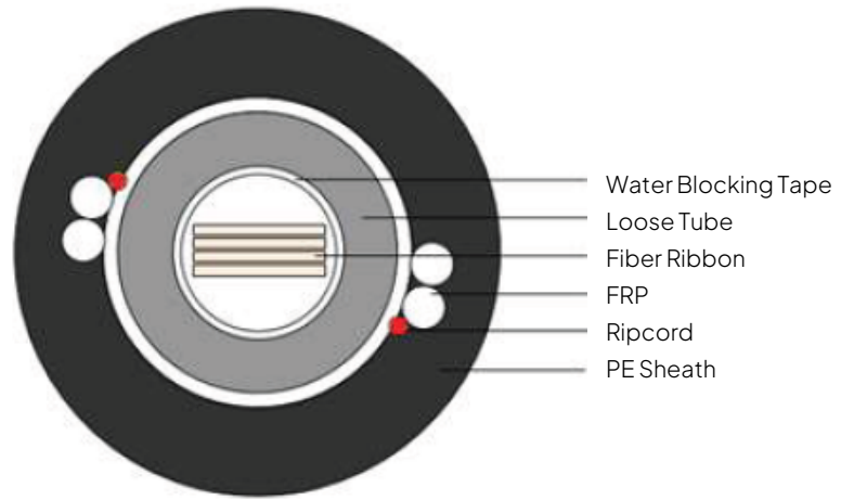
Ribbon SJ/Dielectric (Gel Free) Cable Schematic Purposes Only
